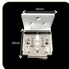
Roller Cassette Brackets
